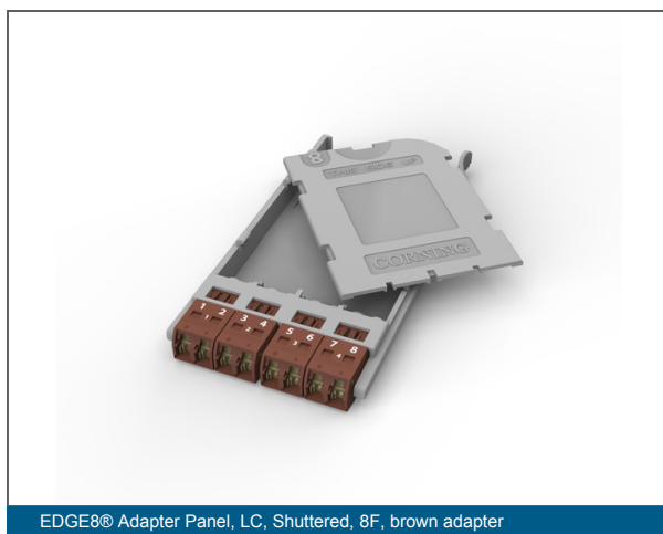
EDGE8® Adapter Panel, LC, Shuttered, 8F, brown adapter
